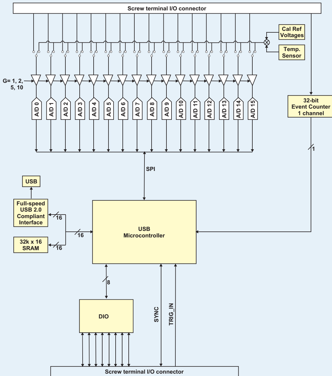
USB-1616FS Block Diagram
